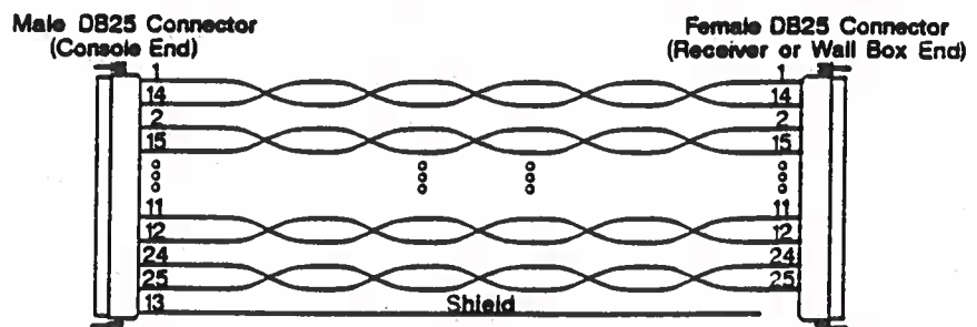
Figure 32. Remote Video Cable
