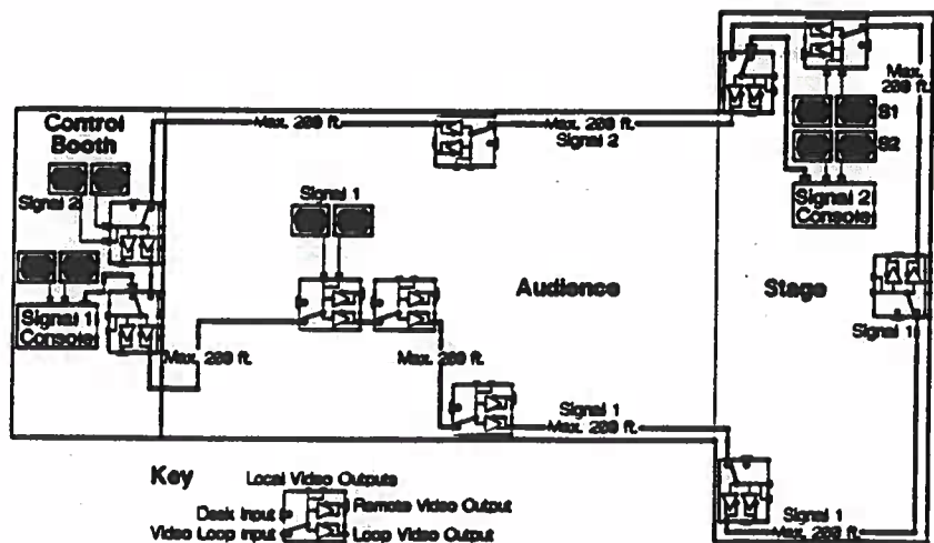
Figure 31. Dual Repeaters for Input and Output
